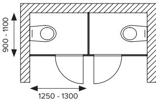
Behinderten WC
