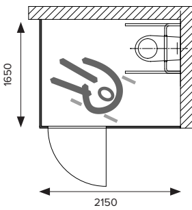
Behinderten WC
